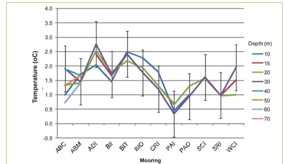
Figure 1 Underwater temperature recorder data averaged over 5 years from SAEONs Algoa Bay thermistor string array
