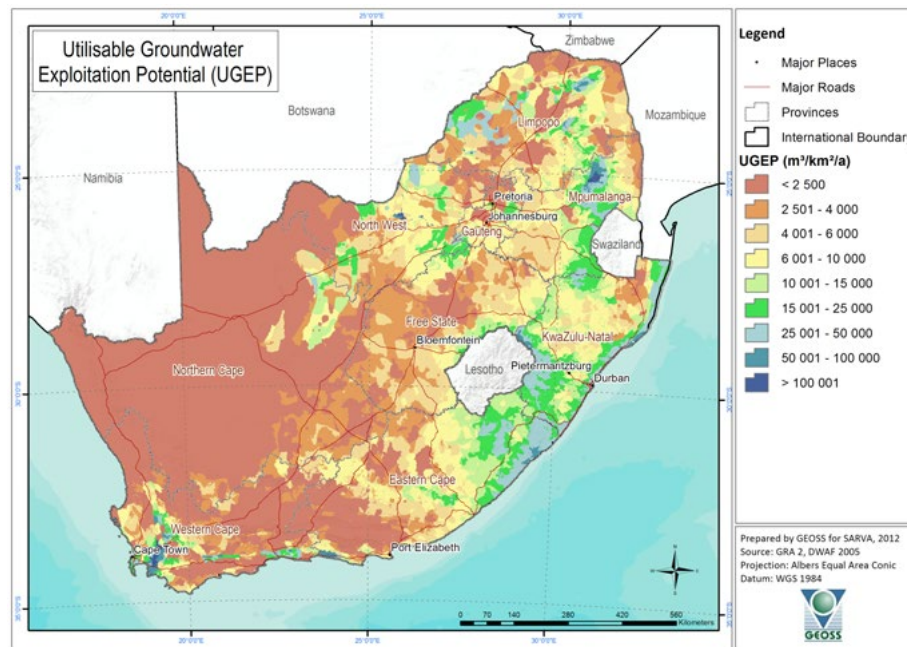
Figure 6.1 Utilisable Groundwater Exploitation Potential (UGEP) for South Africa. (Source: DWAF 2005)
