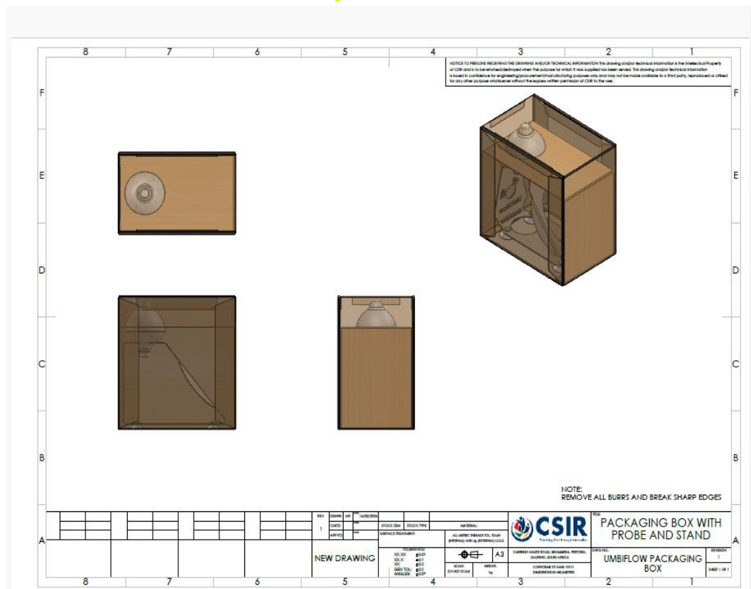
Fig 7: Proposed Design B with Probe and Stand in the box
