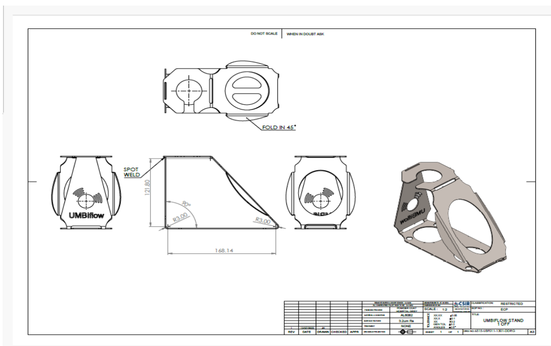
Fig 1: Technical Drawing of the Umbiflow Stand
