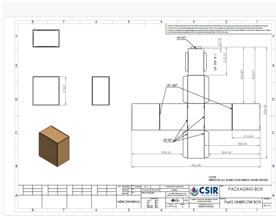
Fig 6: Proposed Design B of the packaging Box
