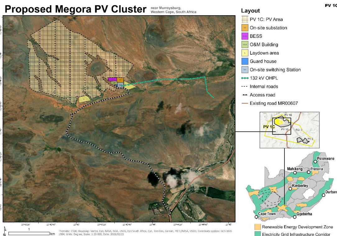
Figure C: Layout of the proposed Megora PV 1C project
