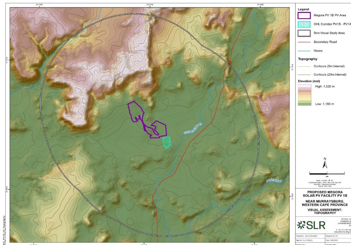
Figure D.4: Topography of the proposed project (Rakale, 2025).
