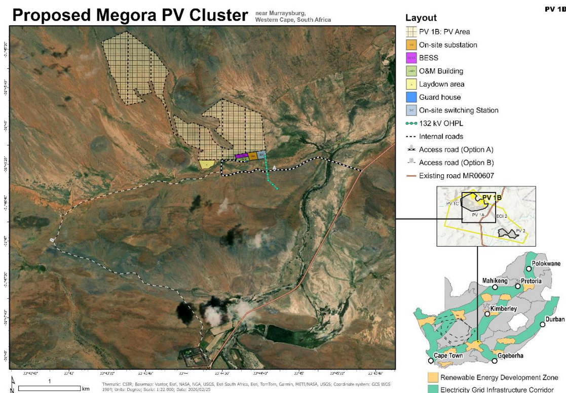
Figure B.1: Project layout of the proposed Megora PV 1 B and associated infrastructure
