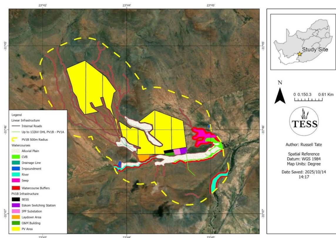
Figure D.12: Layout and aquatic sensitivity map for features within a 500 m radius of the study area showing recommended buffers (Tate, 2025).
