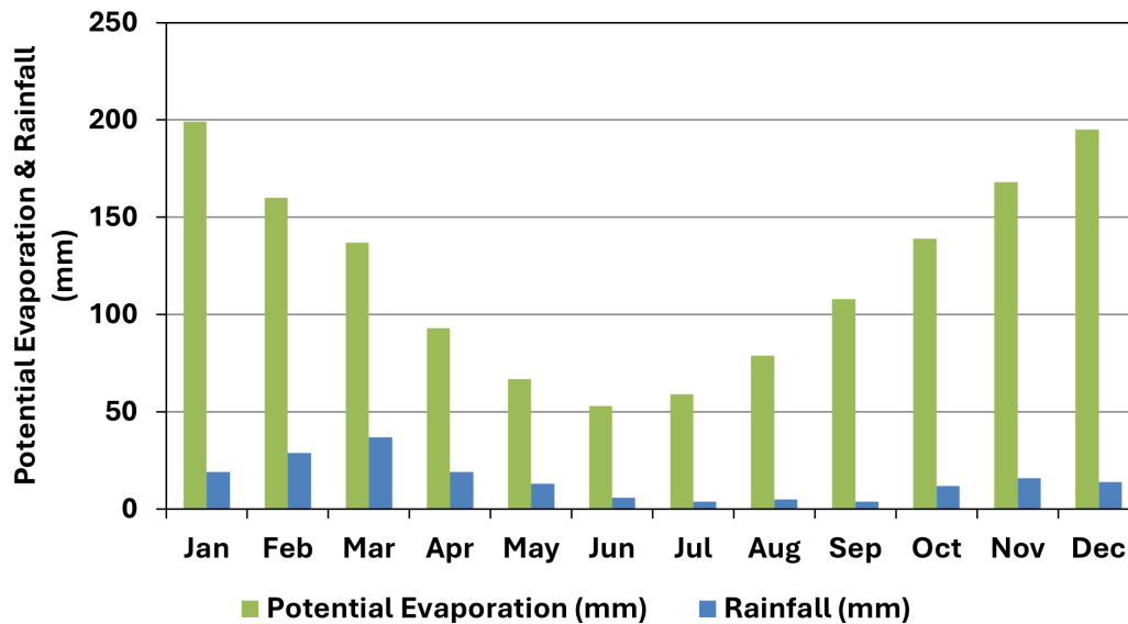
Figure F.2: Monthly average rainfall and evaporation distribution for the study area (Schulze, 2009).
