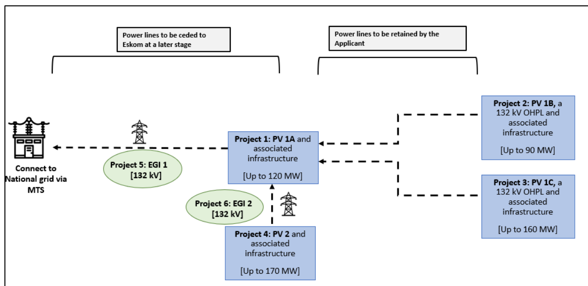
Figure A.1: Summary schematic of the project comprising the proposed Megora Solar PV Cluster
