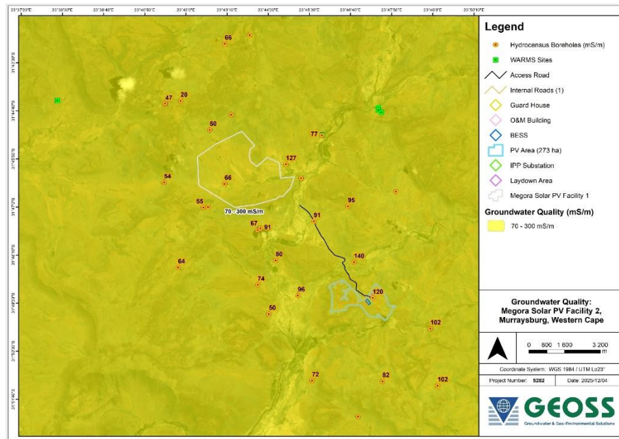
Figure E.6: Regional groundwater quality (mS/m) from DWAF (2005) and borehole groundwater quality (EC in mS/m).
