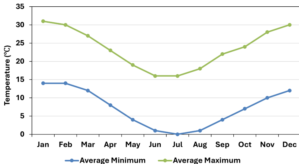
Figure F.1: Monthly average minimum and maximum air temperatures for the study area (Schulze, 2009).
