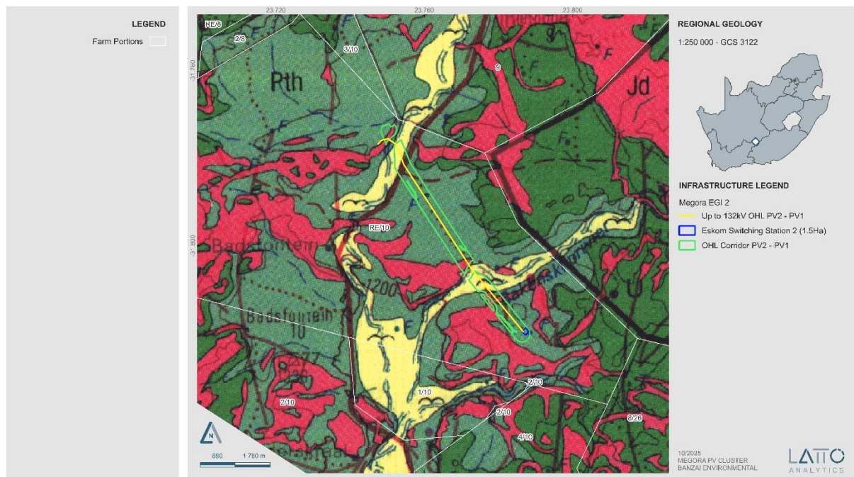
Figure F.3: Regional geological setting of the proposed power line project (3122, Victoria West (CGS, 1984) in Butler, 2025).
