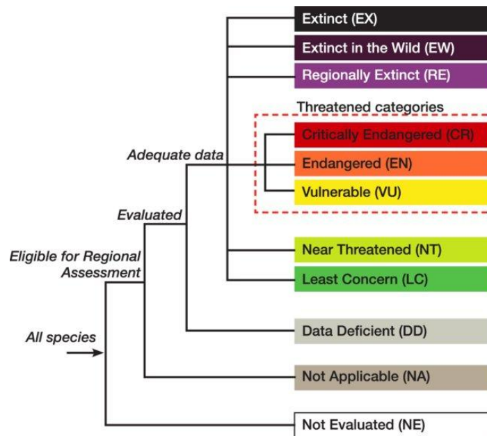
Figure 4: Schematic representation of the structure of the IUCN Red List Categories (IUCN 2012).
