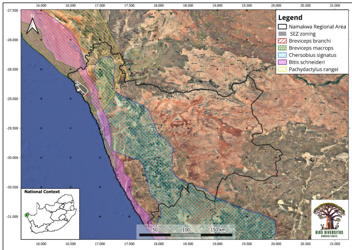
Figure 8: IUCN distribution range for threatened reptile and amphibian species in relation to the Project Area.
