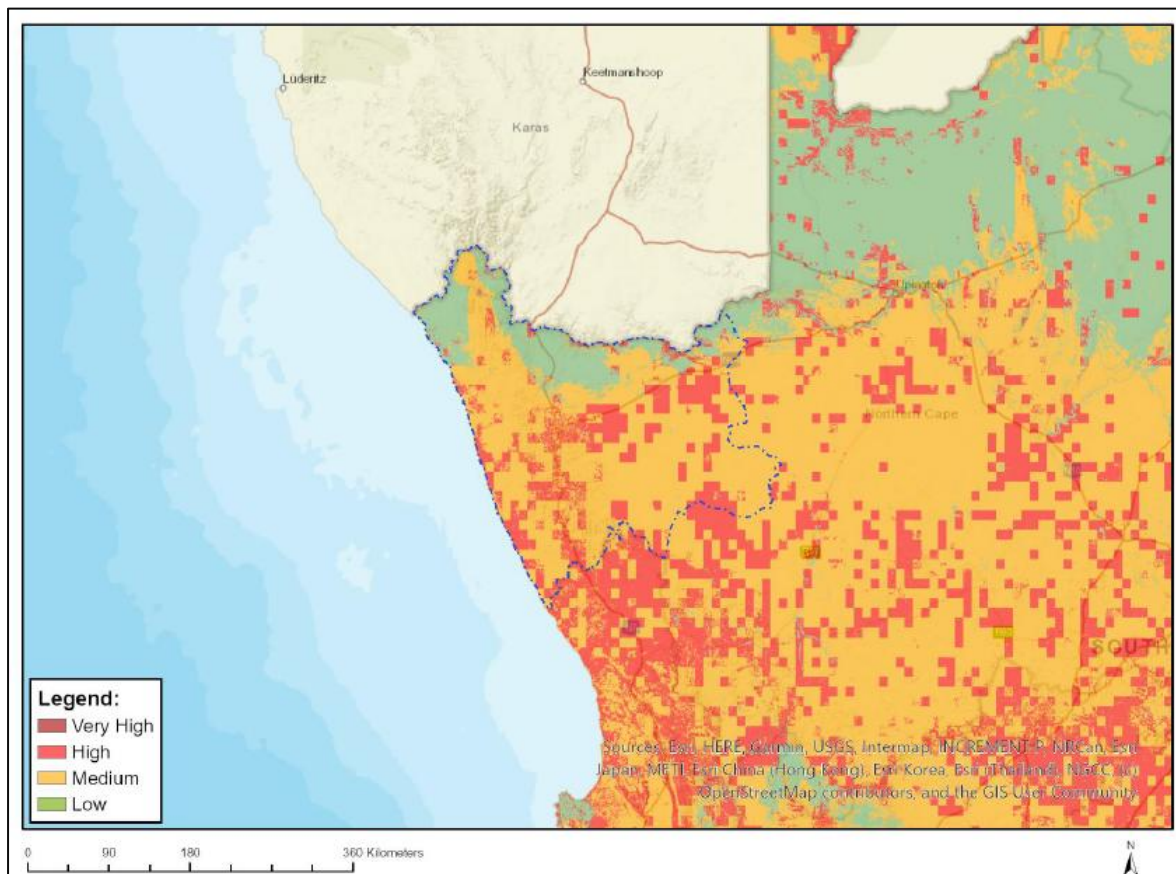
Figure 5: The sensitivity of the Namakwa Region as it relates to the Animal Species Theme (Source: DFFE Screening Tool, 2025).
