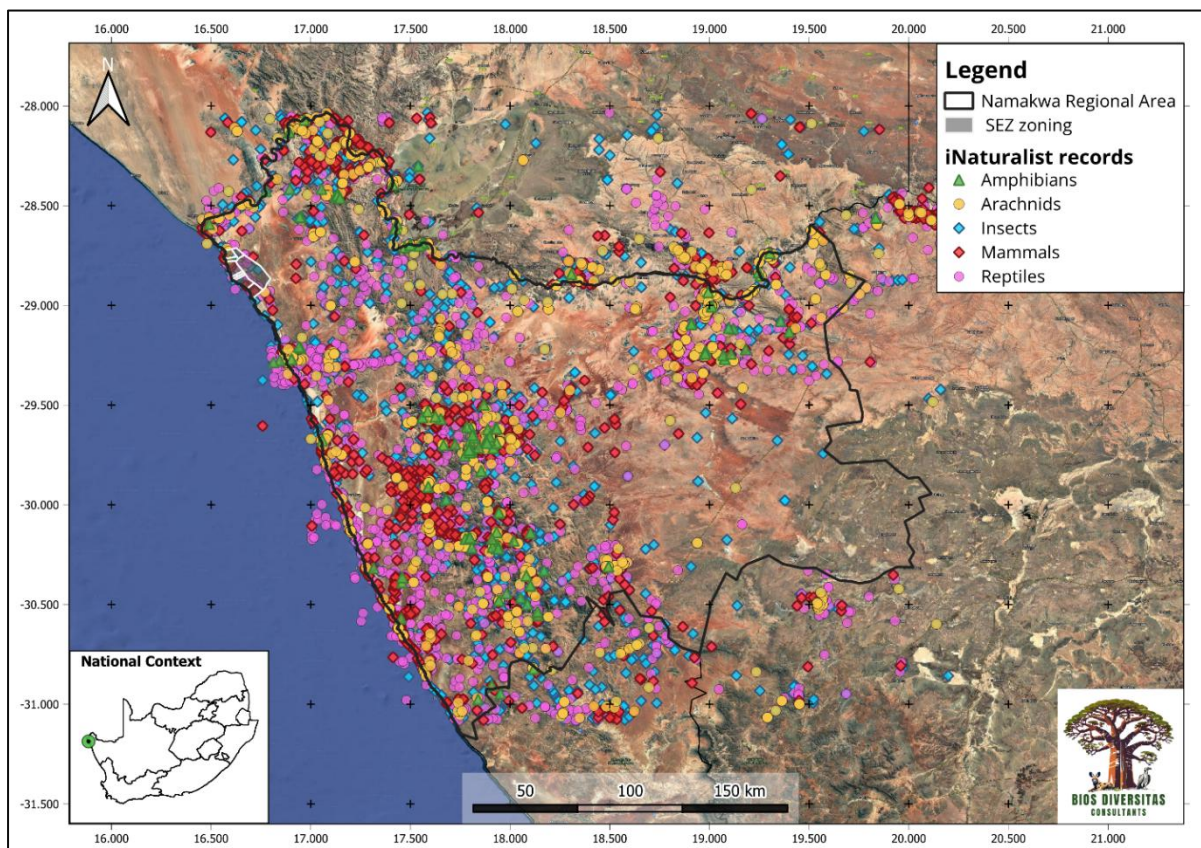
Figure 6: Fauna species records for the regional area (Source: iNaturalist).
