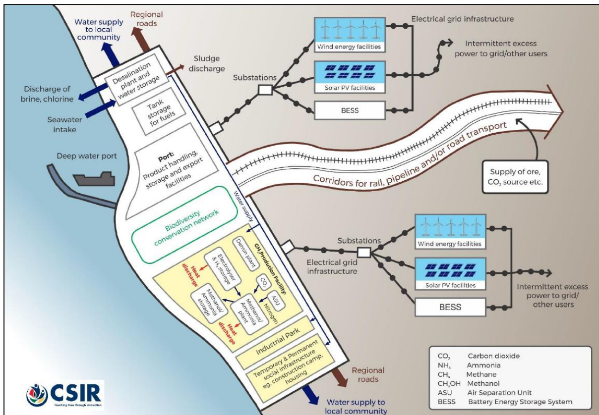
Figure 2: Schematic of the typical main infrastructure components for the Northern Cape regional GH 2 programme (notional drawing, not to scale; source: CSIR briefing note).
