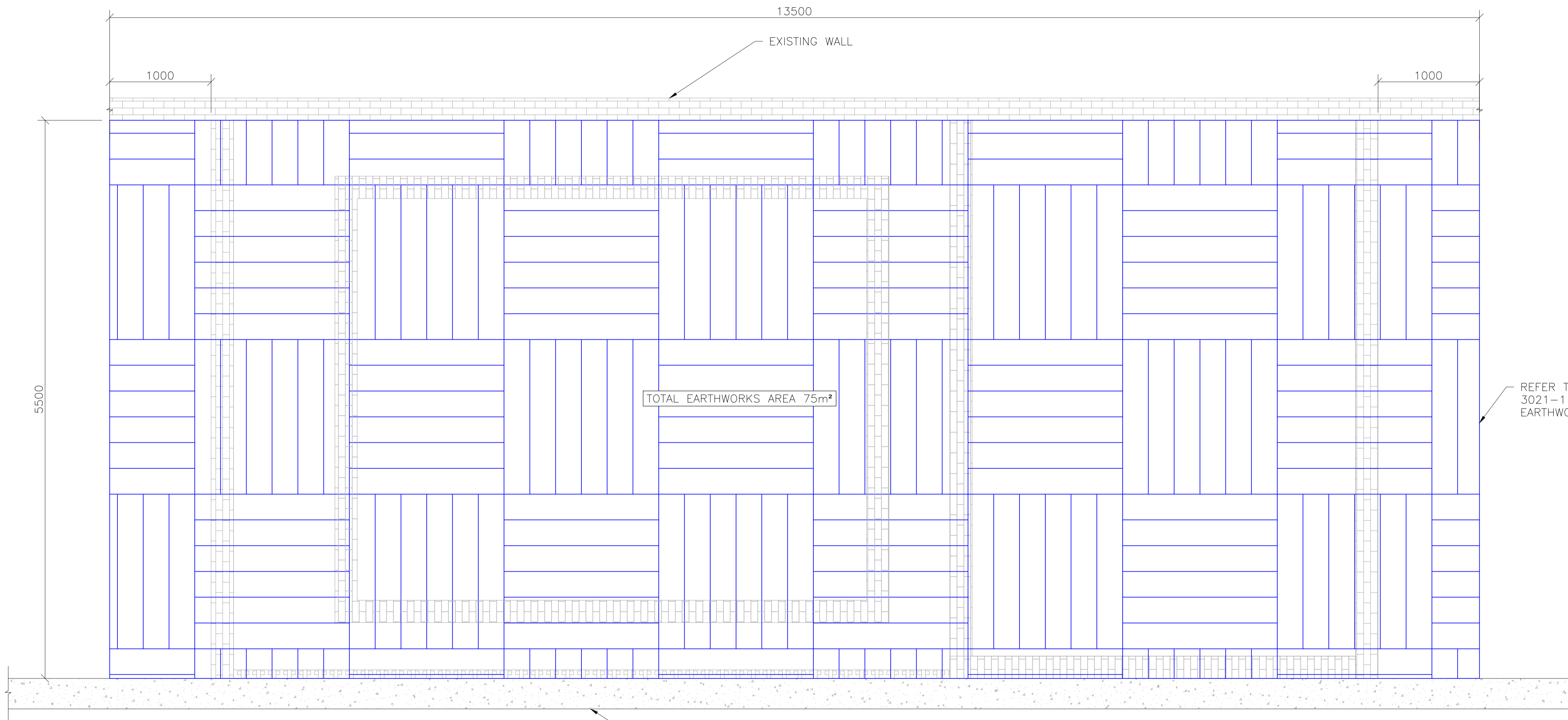
EARTHWORKS LAYOUT SCALE 1:25
