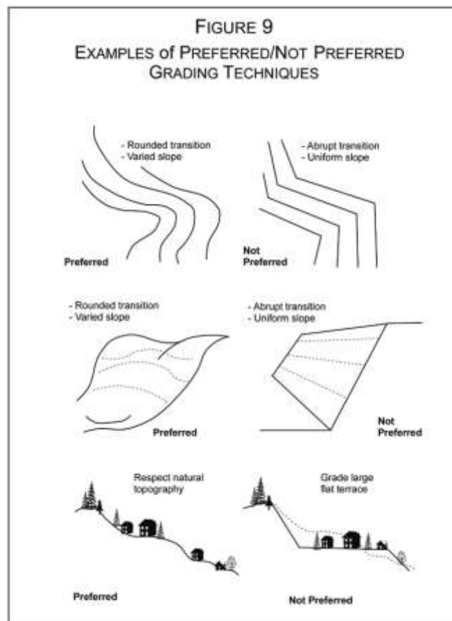
Figure 10-31: Preferred grading techniques ( http://www.lvpc.org/pdf/SteepSlopes.pdf )
