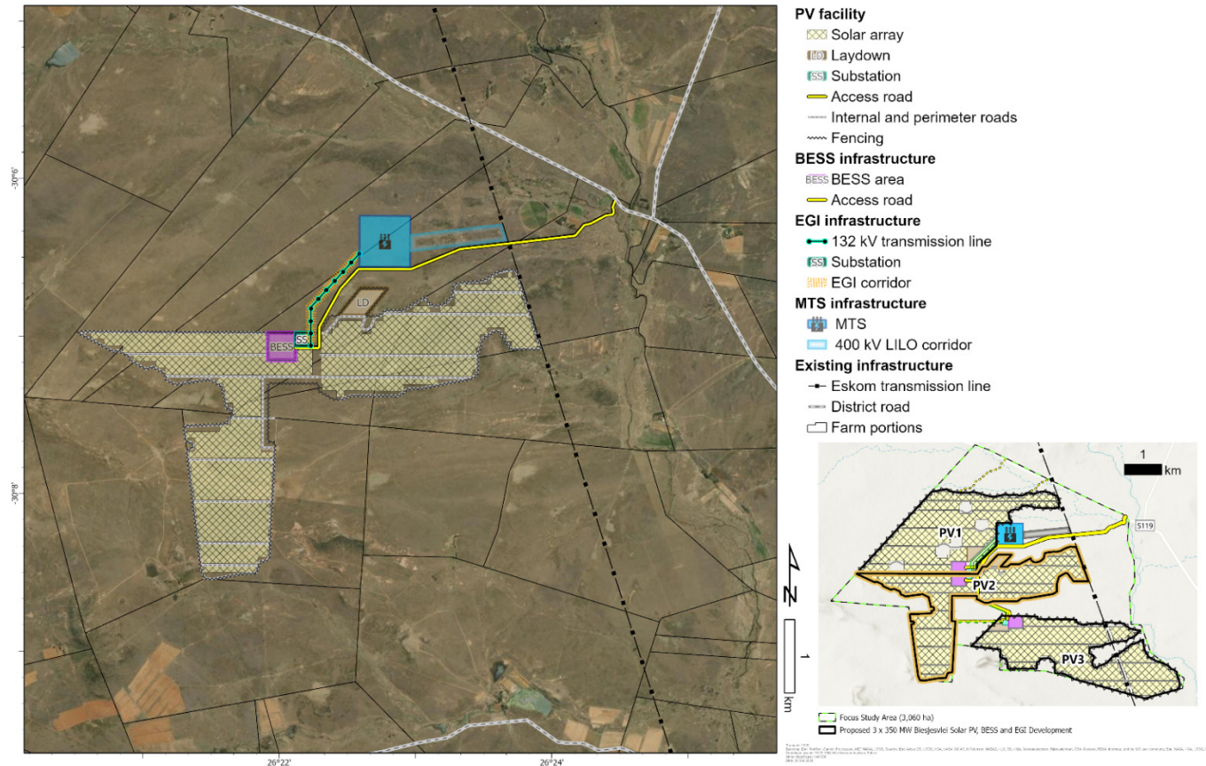
Figure 7.6: Preliminary Project Layout for Project 2 (Biesjesvlei PV2), Project 5 (Biesjesvlei BESS 2), and Project 8 (Biesjesvlei EGI 2) [including Project 10 (Biesjesvlei MTS and LILO)]
