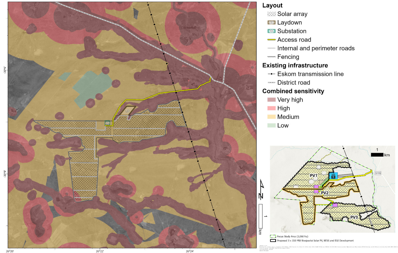
Figure 7.7: Combined Preliminary Project Layout and Sensitivity Map for Project 2 (Biesjesvlei PV2)
