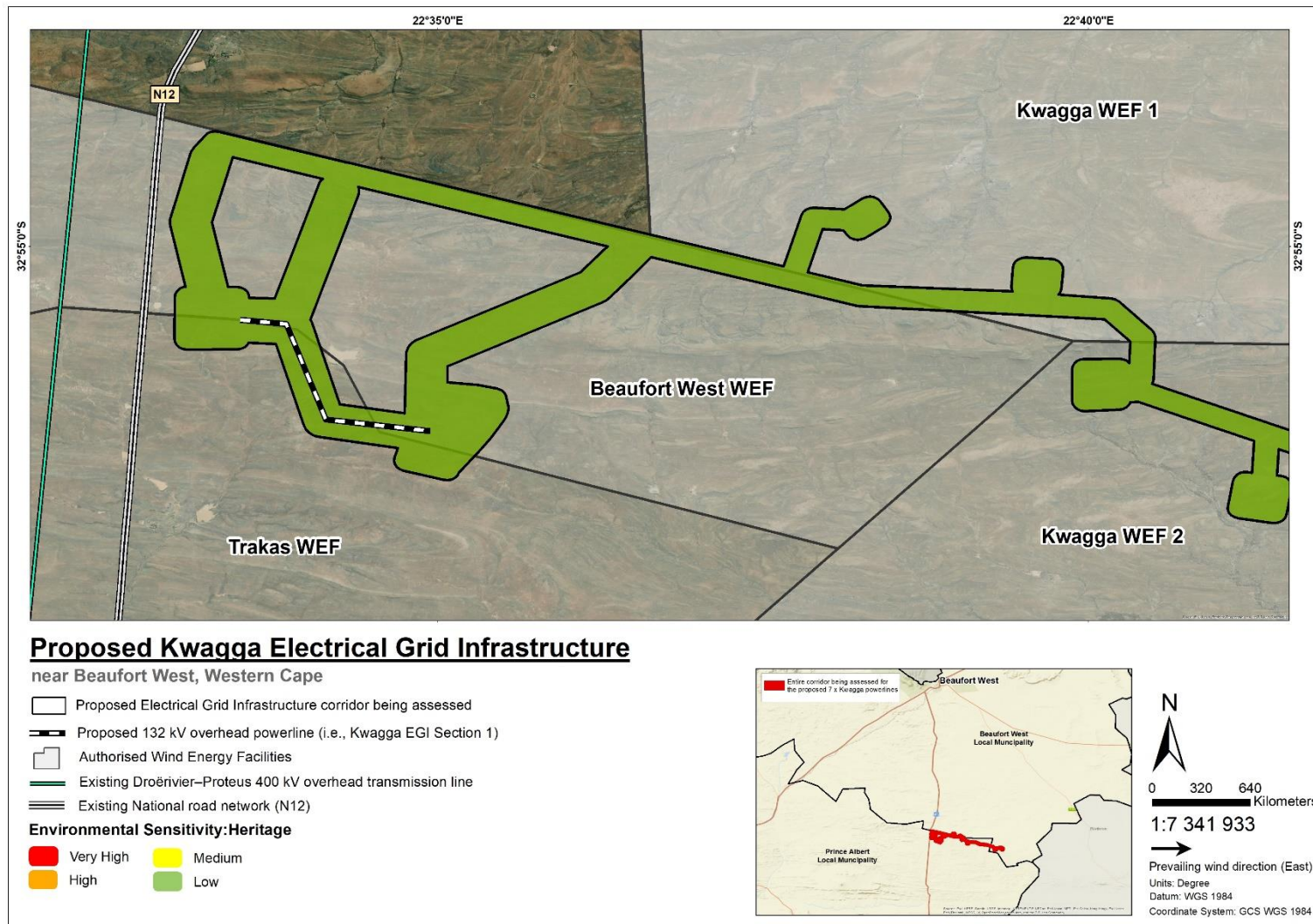
Figure C.9: Heritage sensitivity map for the proposed 132 kV overhead powerline i.e. Section 1 of the Kwagga EGI corridor, which extends between the proposed authorised Beaufort West 132 kV-400 kV Linking Station and the Eskom 132 kV Switching Substation.
