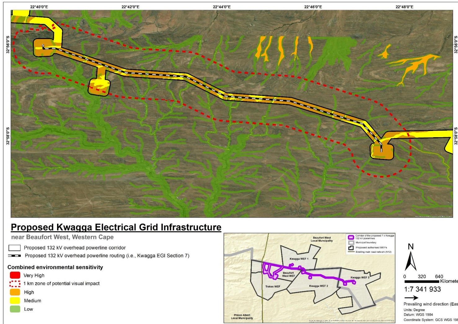
Figure 5. Combined environmental sensitivity map for the proposed 132 kV overhead powerline i.e. Section 7 of the Kwagga EGI corridor, which extends between the proposed authorised on-site substation hubs at the Kwagga WEF 3 site and the Kwagga WEF 2 site
