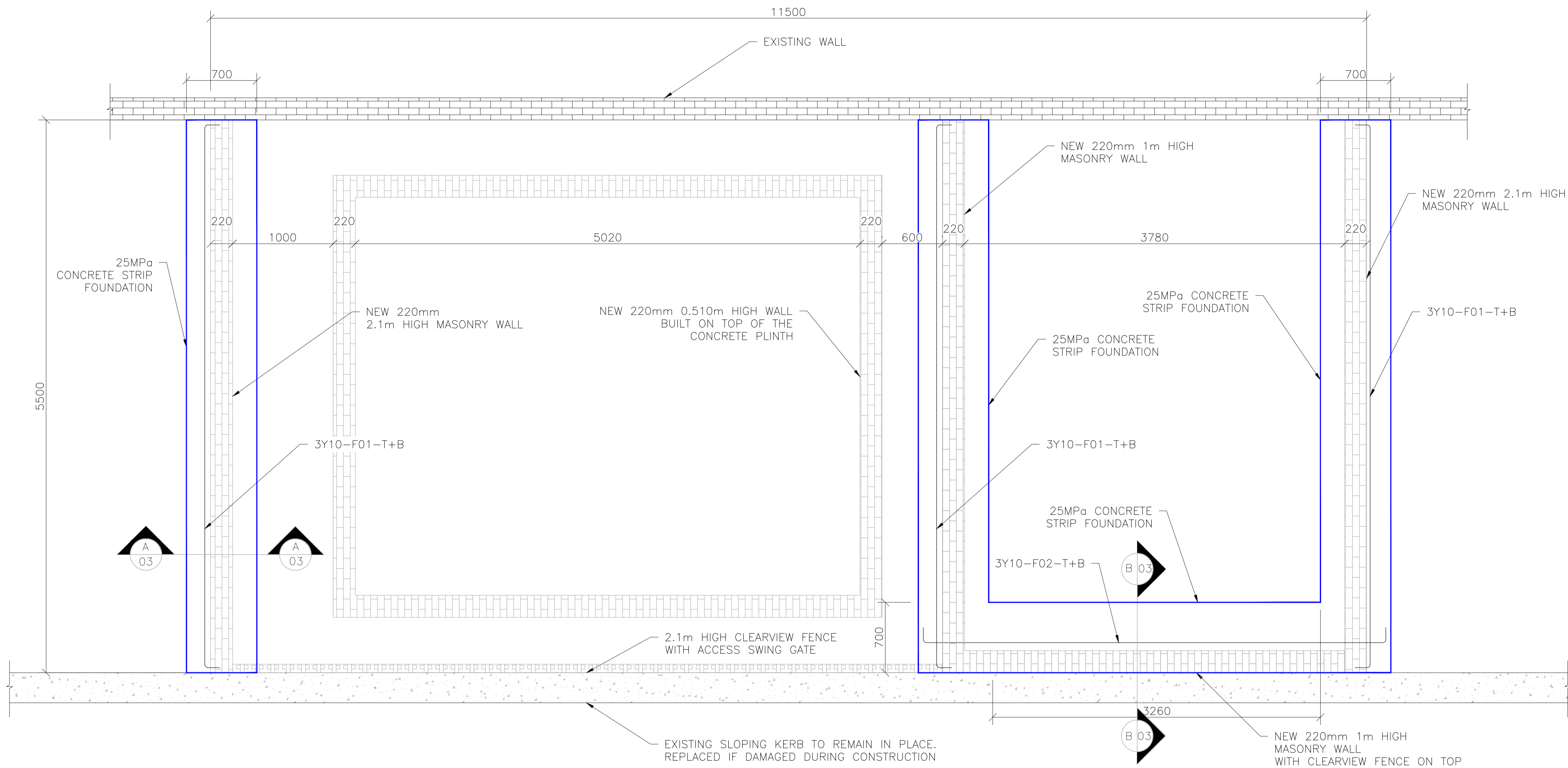
STRIP FOUNDATION LAYOUT SCALE 1:25
