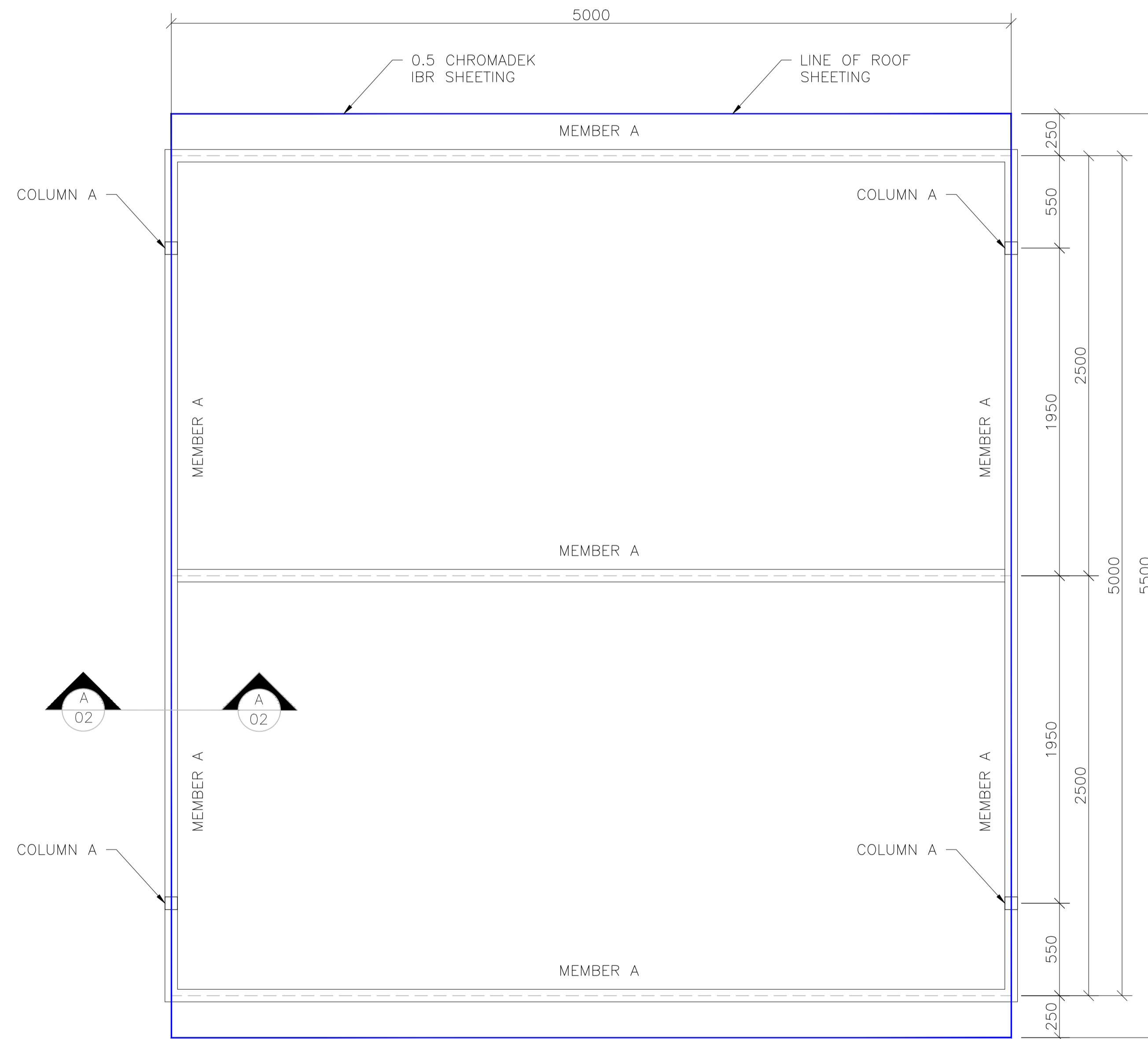
PLAN VIEW SCALE 1:20
