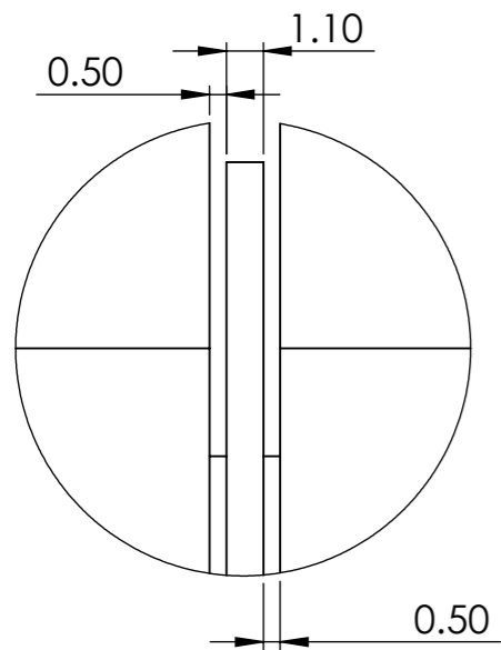
DETAIL B SCALE 4 : 1
