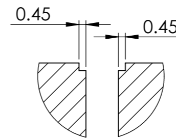
DETAIL E SCALE 4 : 1
