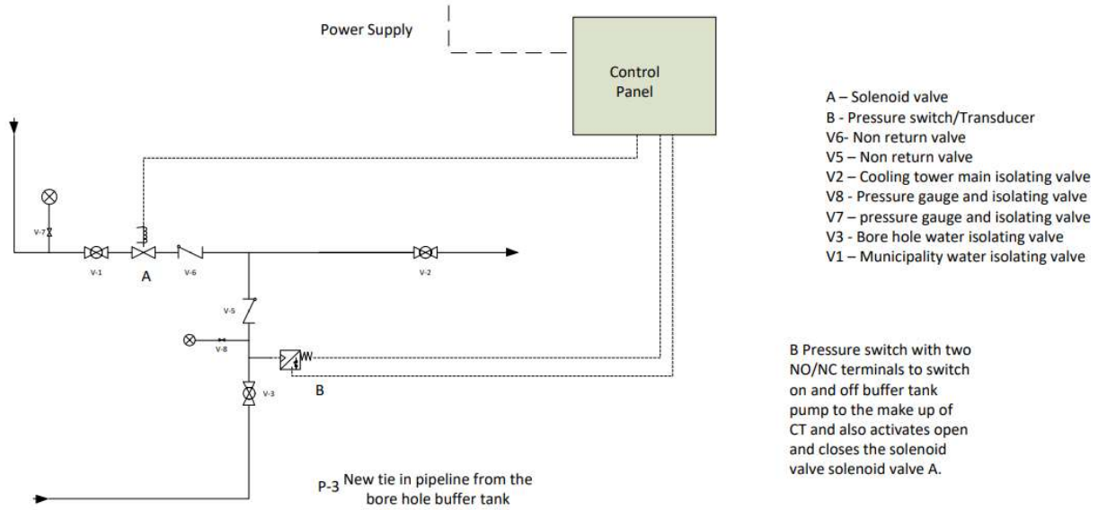
Figure 1: Borehole make-up to cooling tower control system
