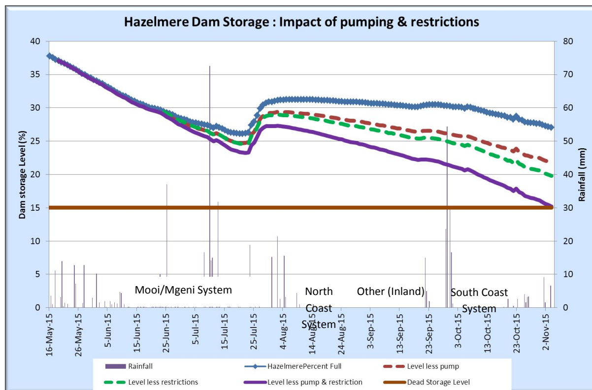
Figure 1-5 Impact of pumping from the Mpambanyoni River on EJ Smith Dam (Umgeni Water, 2015)
