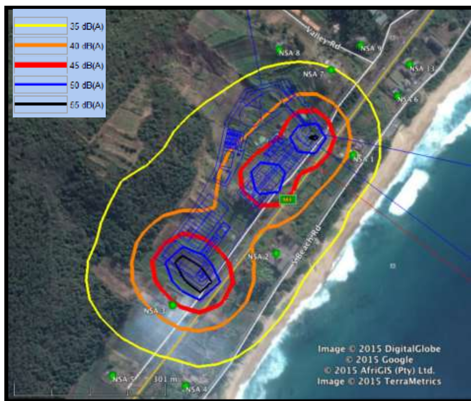
Figure 9-6 - Operational Phase – Main Plant Noise Impact
