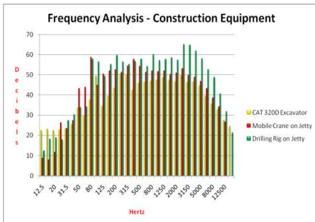
Figure 9-5 – Frequency Analysis for a selection of construction equipment
