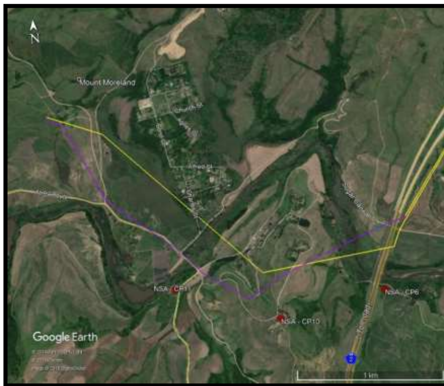
Figure 9-4: Aerial image indicating proposed powerline routes to be constructed to serve the desalination plant (Yellow: Proposed powerline route, Purple: Realignment of the original Proposed powerline route).
