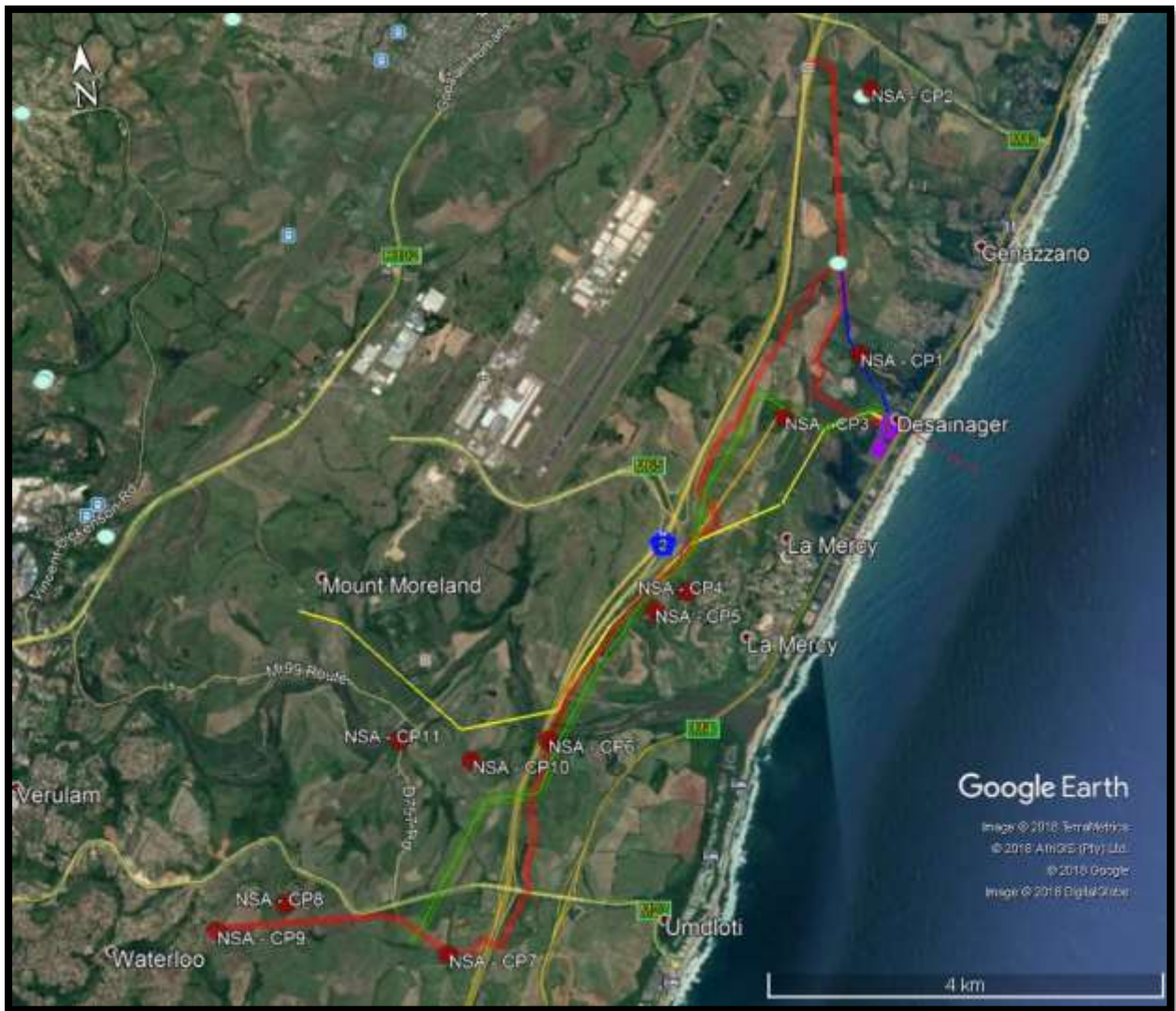
Figure 9-3 - Map of the proposed pipeline (Original route = blue; Proposed pipeline Alternative 1 (Red)) and powerline (yellow (Proposed route); orange (Alternative 1 route) and green (Alternative 2 route)) showing noise sensitive receptors
