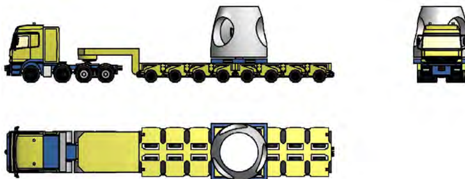
Figure 13: Transporting the Hub and Rotary Units
