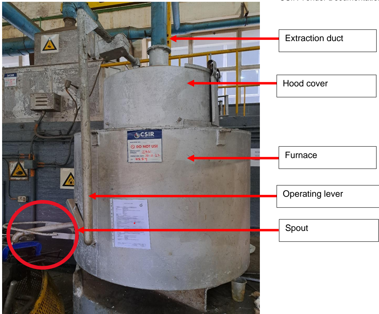
Fig 1: Furnace
