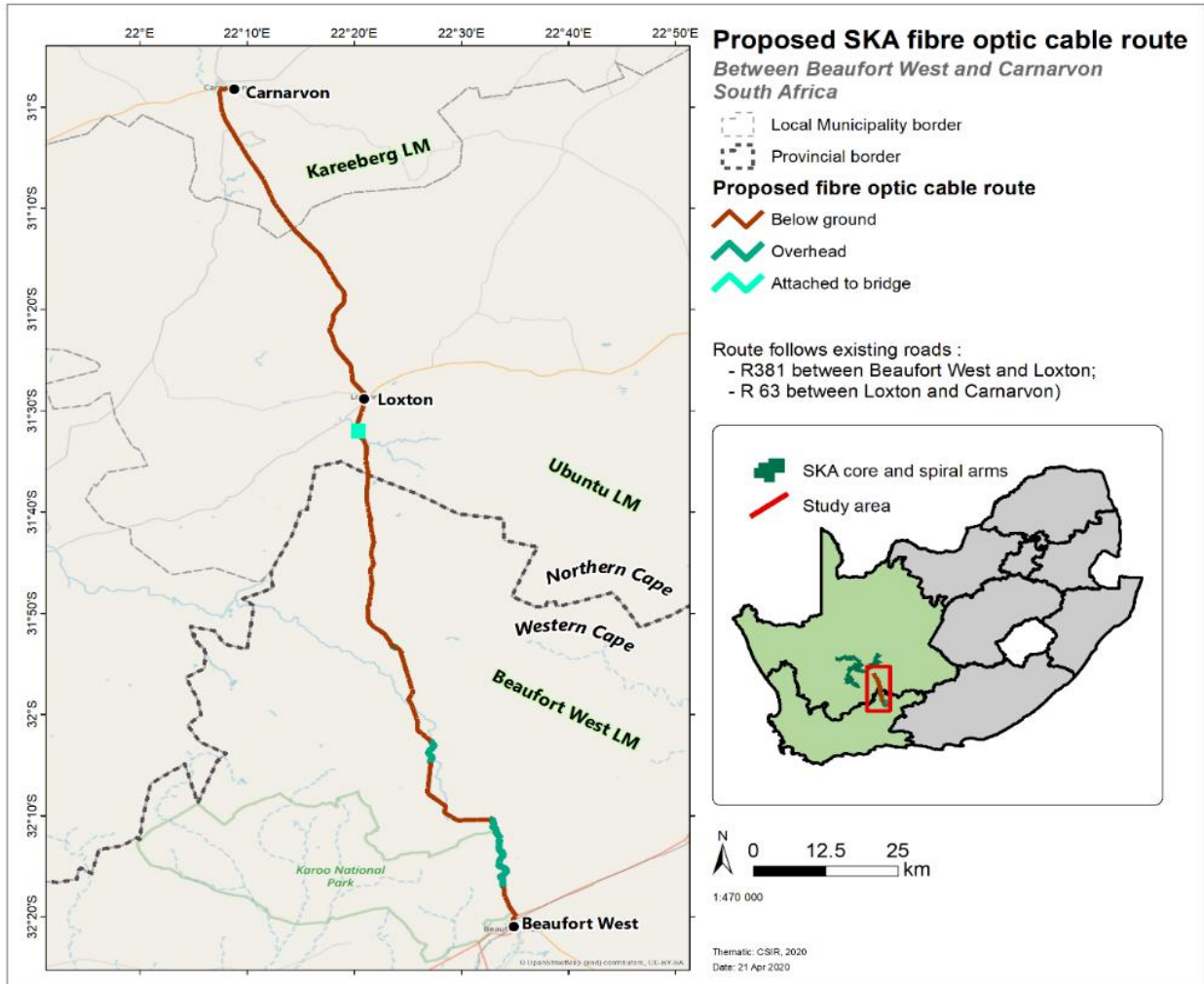
Figure 1: The proposed SKA fibre optic cable route starts in Beaufort West, follows the existing R 381 and R 63 roads via Loxton to Carnarvon. Note Overhead and underground distance may change
