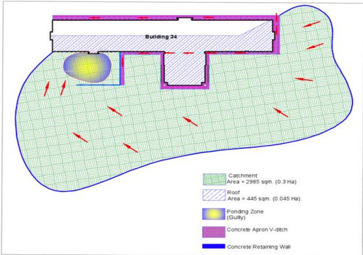
Building 34 - Catchment area and ponding zone
