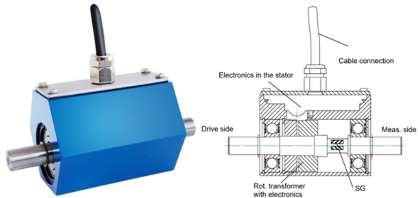
Figure 8.7: DR-2477 non-contact precision torque sensor with a rotary operational principle [25]
