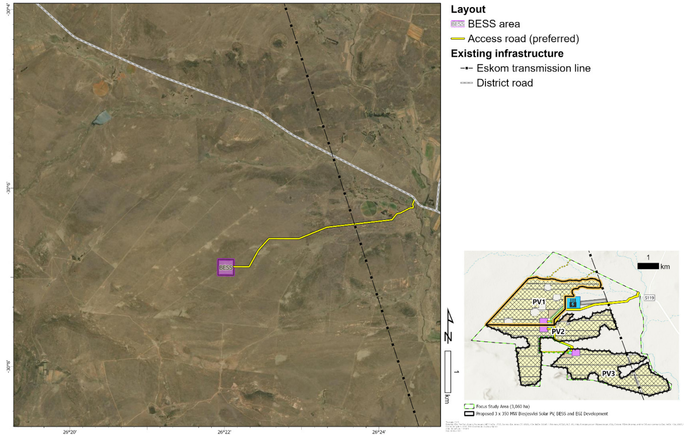
Figure 7.4: Preliminary Project Layout Map for Project 4 (Biesjesvlei BESS 1)
