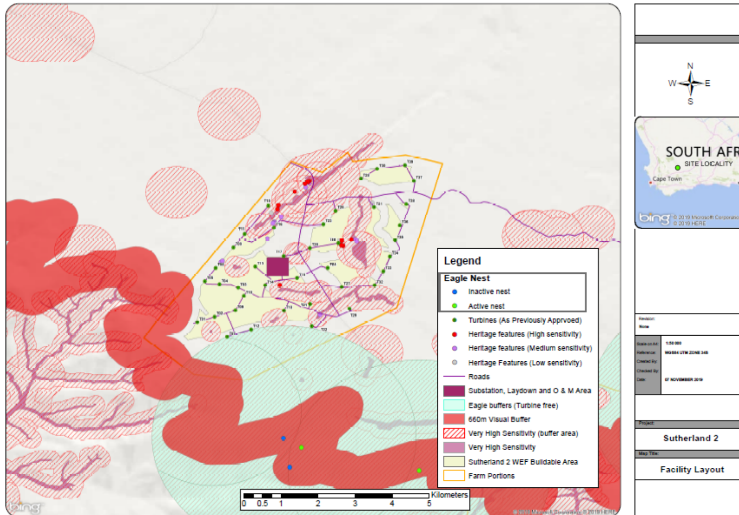
Figure 14: Environmental sensitivity map overlay with the turbine locations for the Sutherland 2 WEF (illustrating the Verreaux's Eagle nests)
