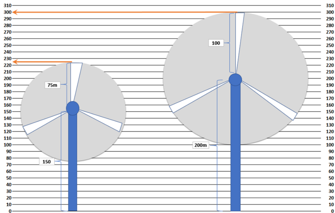
Figure 5: Changes in specifications of turbine dimension
