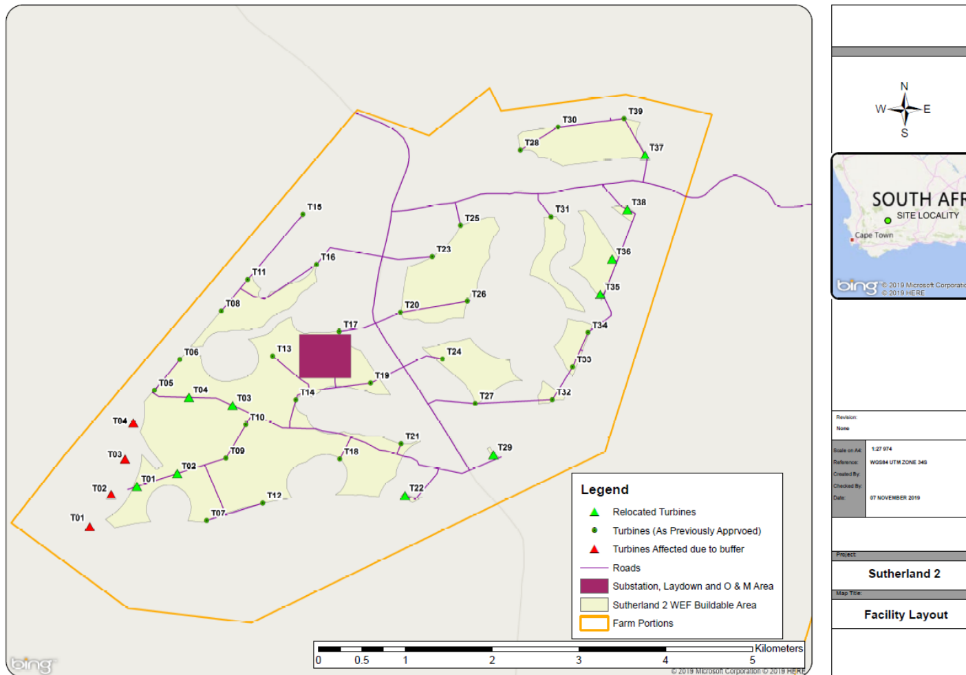
Figure 1: Locality map illustrating the authorised turbines and relocated turbines
