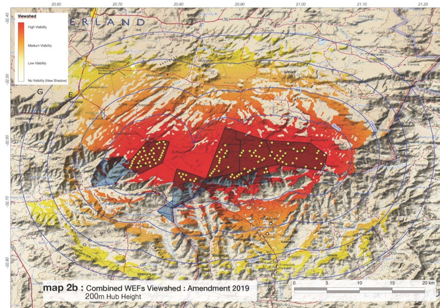
Figure 9: Combined WEFs (Rietrug, Sutherland, Sutherland 2) viewshed: Amendment 2019: 200 m Hub Height (Oberholzer and Lawson, 2019).
