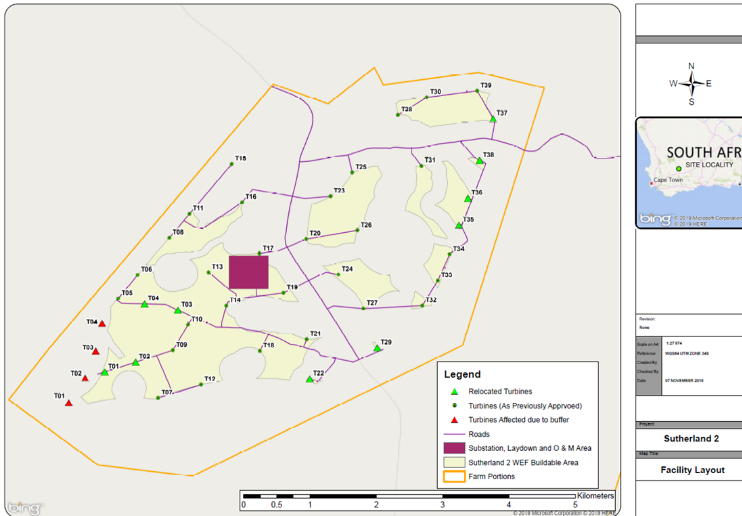
Figure 11: Authorised layout and amended layout of the proposed Sutherland 2 Wind Energy Facility
