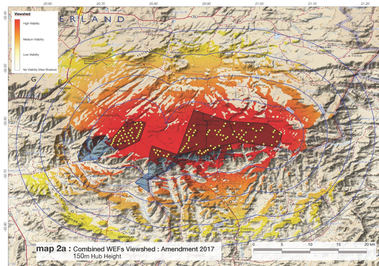
Figure 8: Combined WEFs (Rietrug, Sutherland and Sutherland 2) viewshed: Amendment 2017: 150 m Hub Height (Oberholzer and Lawson, 2019)
