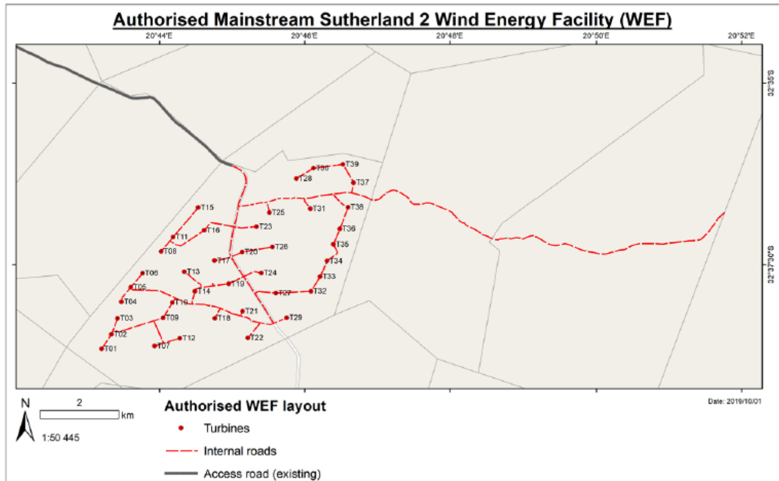
Figure 3: Approved layout for the Sutherland 2 WEF as per the Environmental Authorisation obtained in 2016
