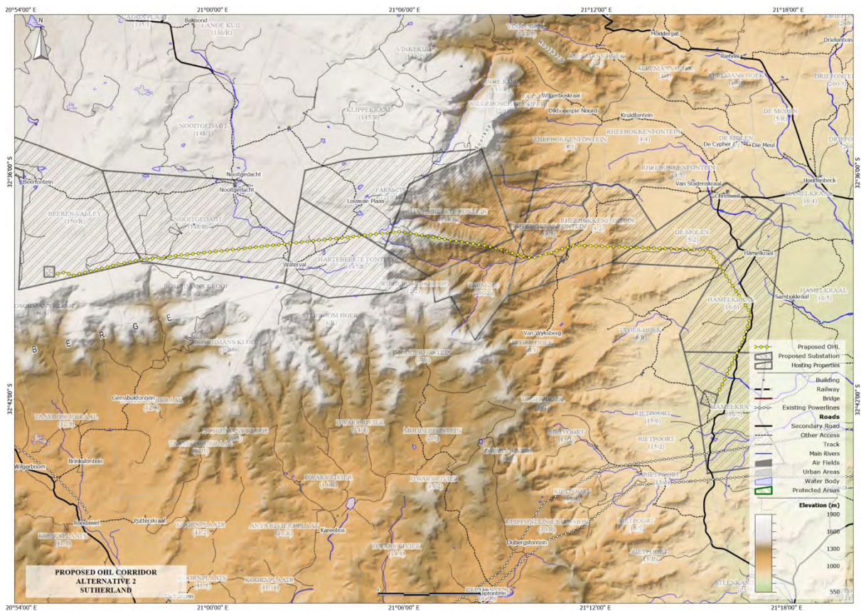
Figure 1-2 Proposed Alternative 2 132 kV overhead line and substations associated with the Sutherland WEF.
