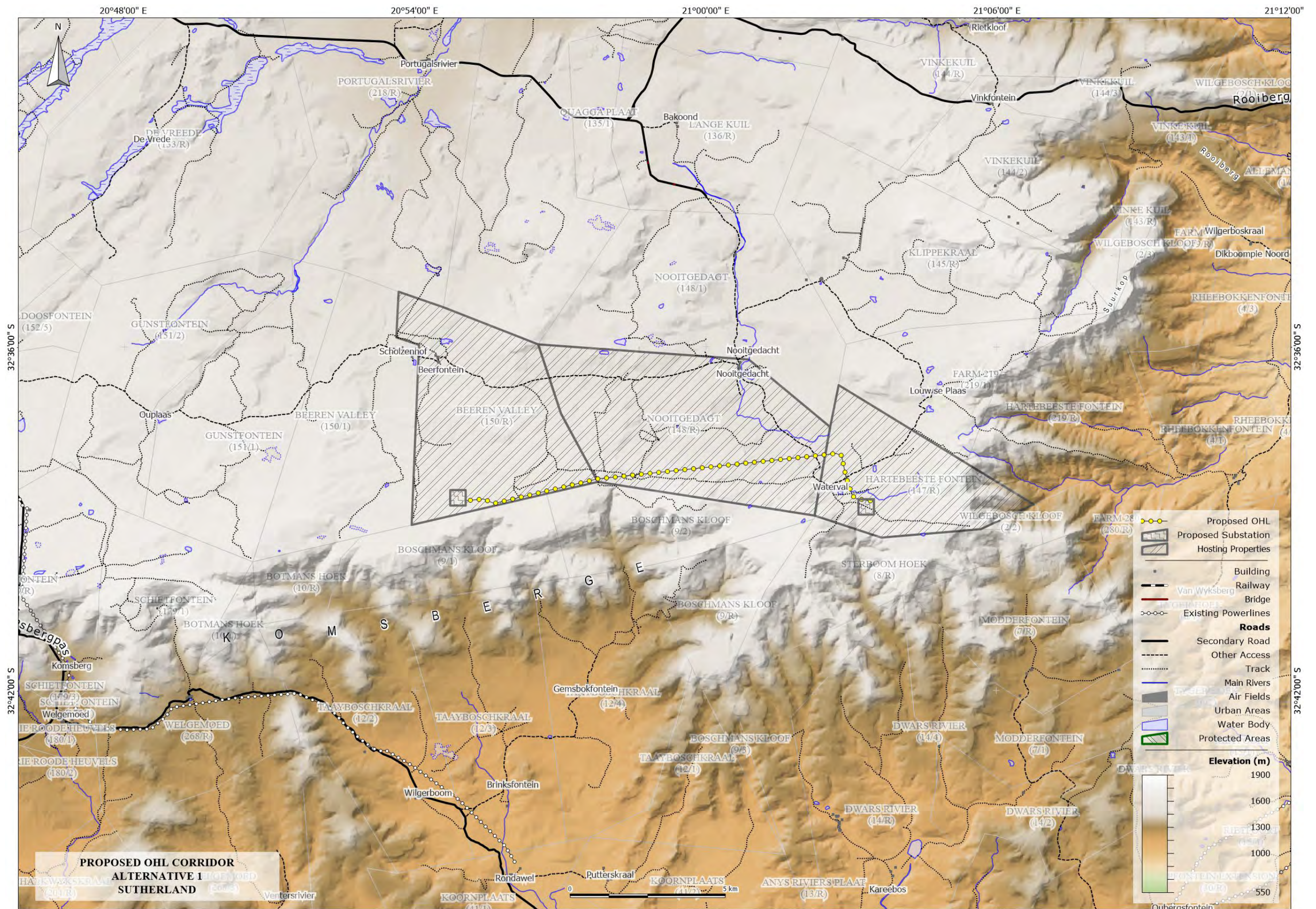
Map 1 Proposed Alternative 1 of the 132 kV overhead line and substations associated with the Sutherland WEF.
