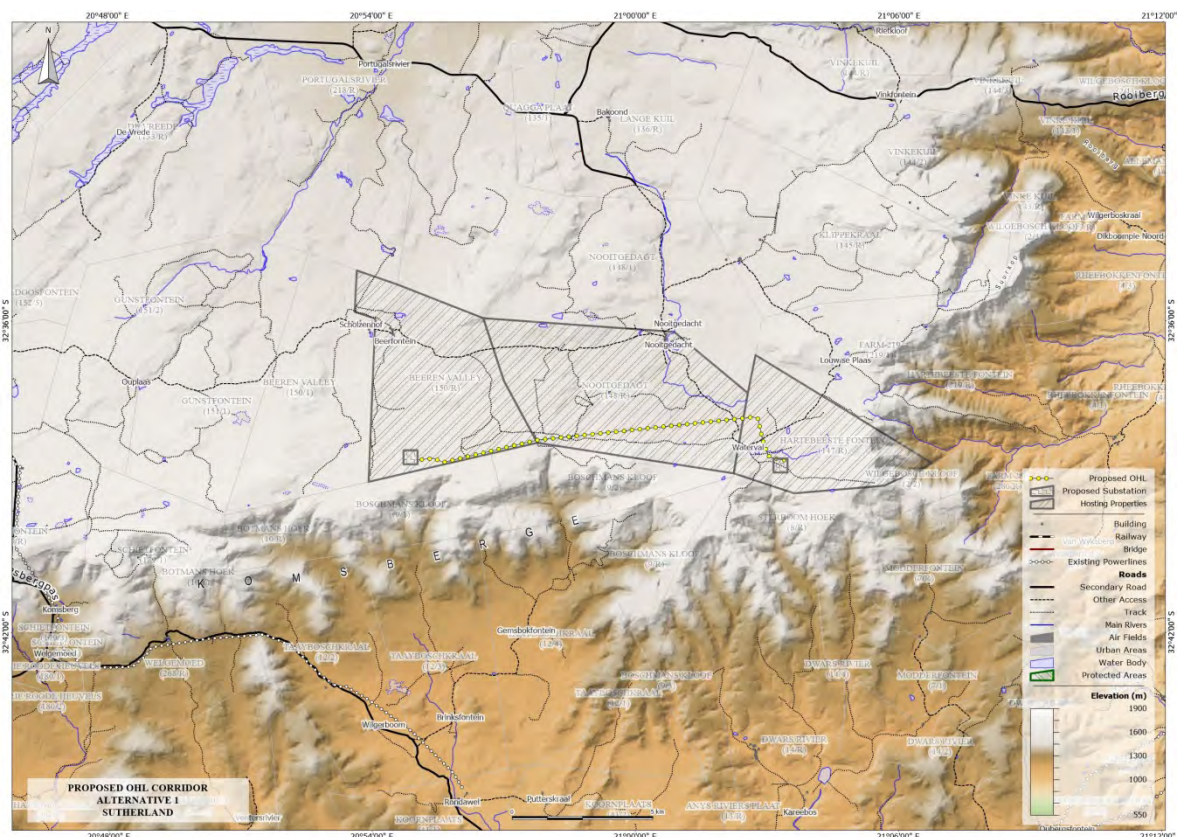
Figure 1-1 Proposed Alternative 1 132 kV overhead line and substations associated with the Sutherland WEF.
