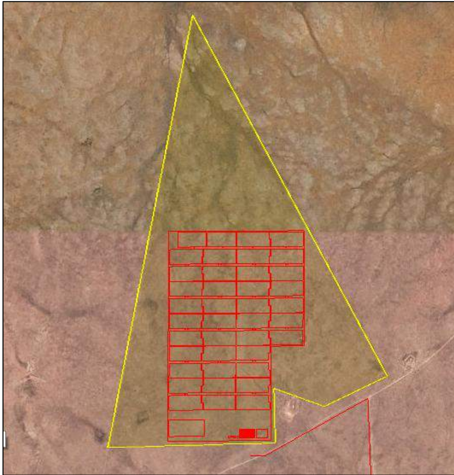
Figure 9. The detailed Skeerhok PV 1 layout superimposed on Google Earth image. The developable area is shown in yellow and the actual layout footprint in red.
