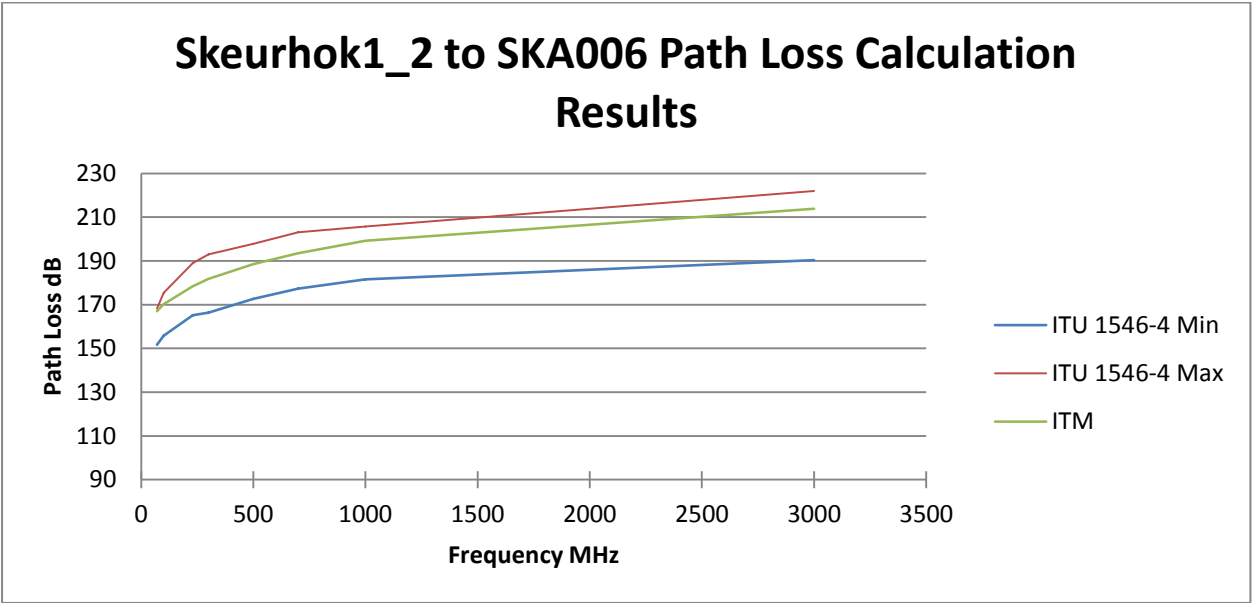
Graph 2: Skeurhok 1_2 to SKA006 Path Loss Calculation Results
