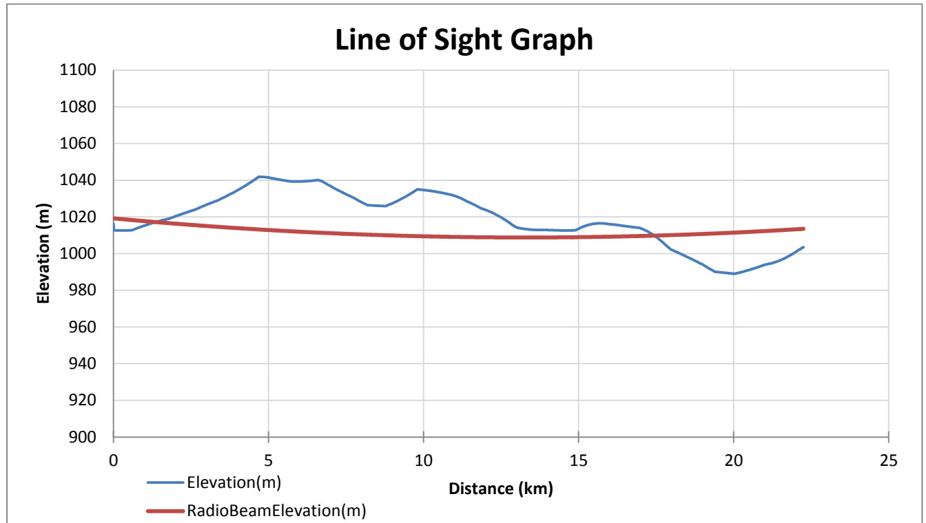
Figure 8: Skeurhok 1_2 to SKA ID 2366
