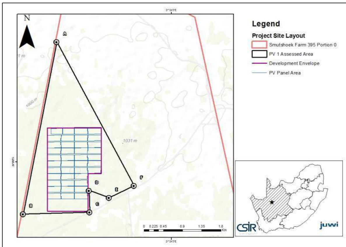
Figure 1. The position and layout of the proposed Skeerhok PV 1 facility.
