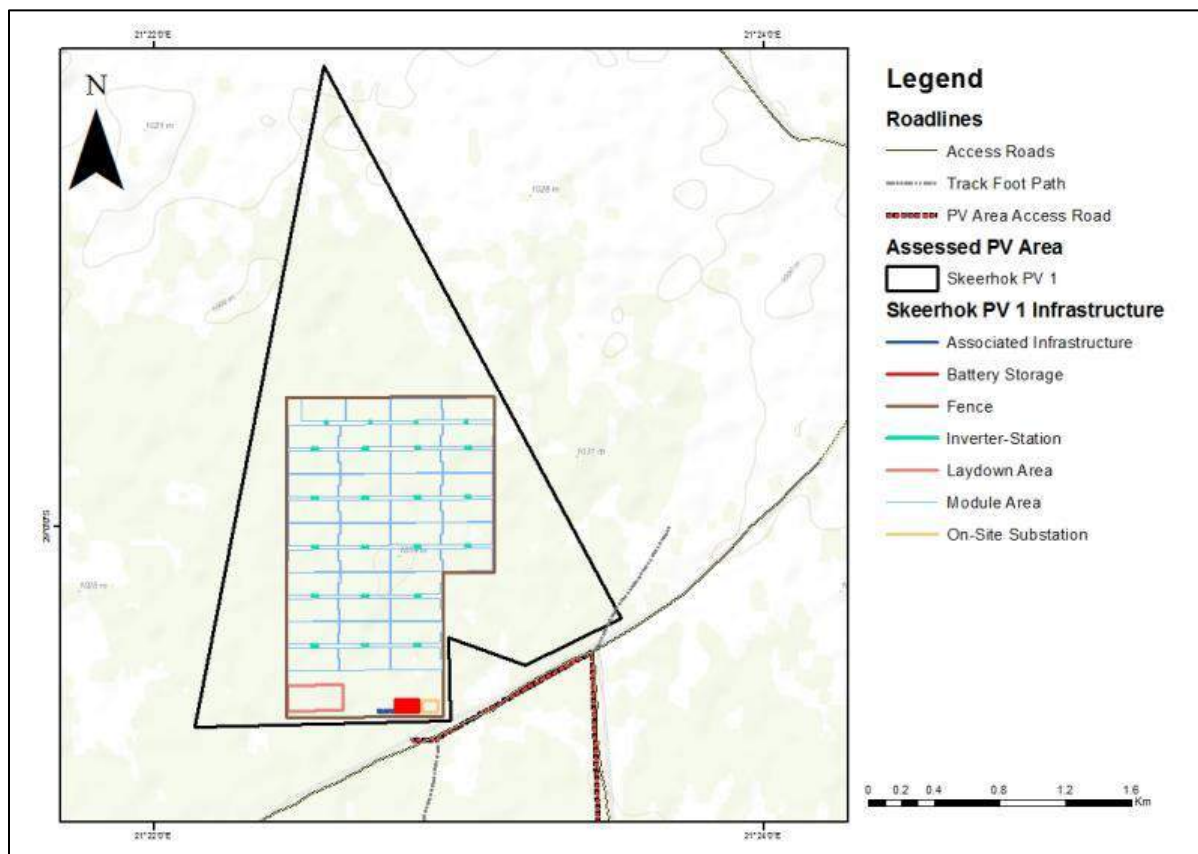
Figure 2. Proposed layout of the Skeerhok PV 1 facility.
