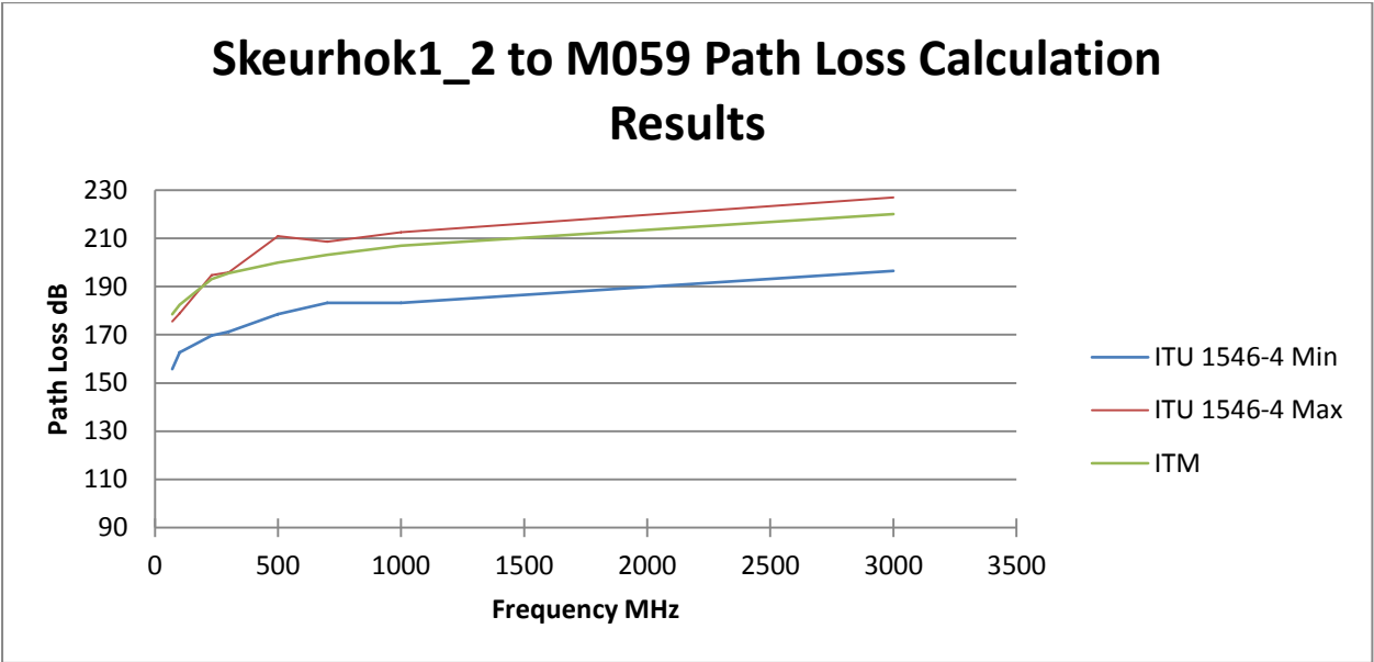
Graph 1: Skeurhok 1_2 to M059 Path Loss Calculation Results
