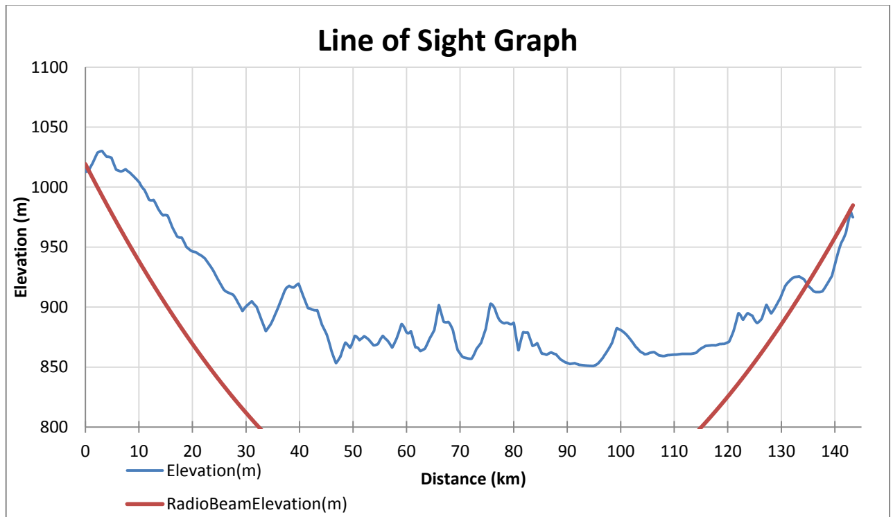
Figure 7: Skeurhok 1_2 to SKA ID 006
