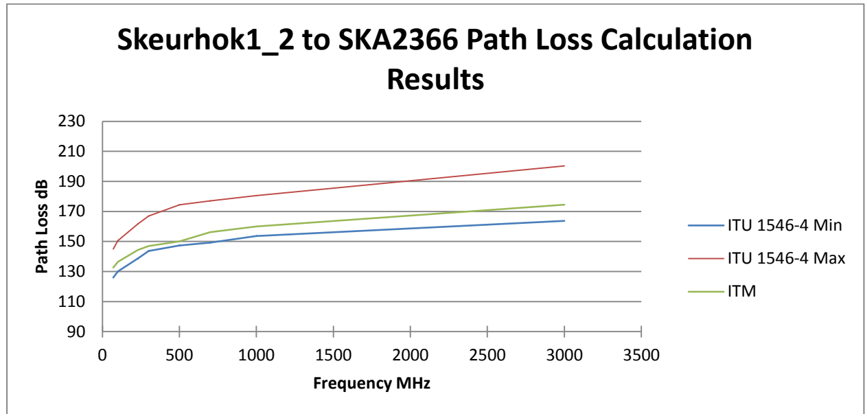
Graph 3: Skeurhok 1_2 to SKA2366 Path Loss Calculation Results
