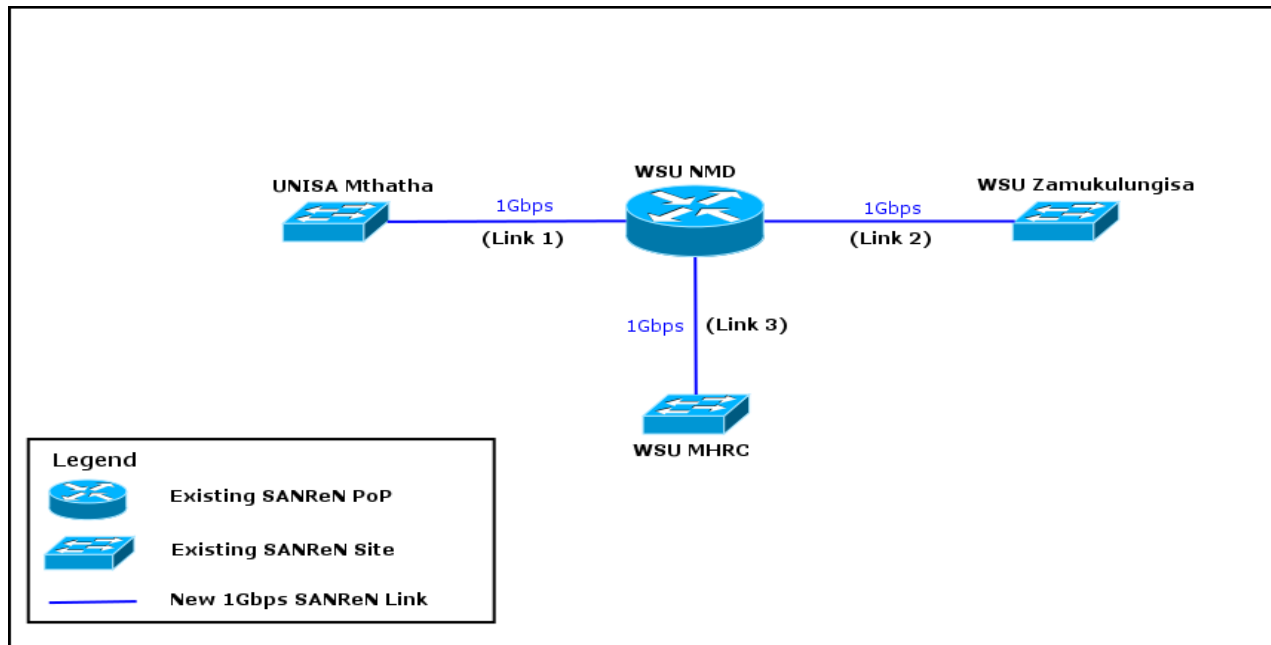
Diagram 1: Schematic diagram of managed bandwidth links between Mthatha Links
